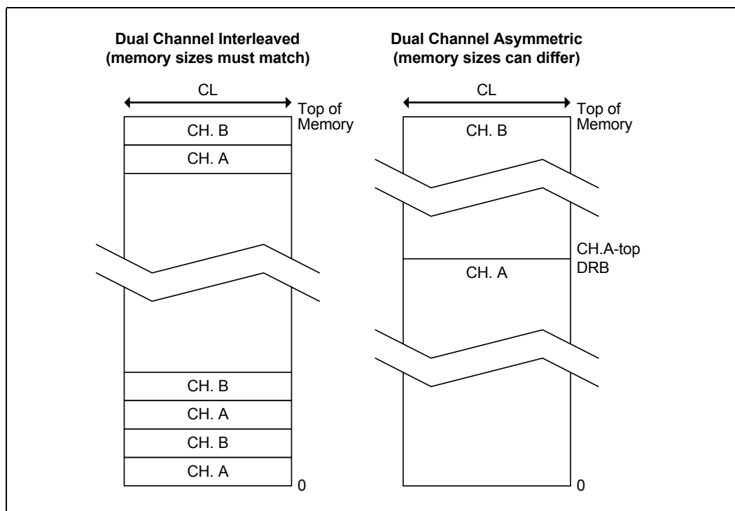
Figure 2-2. Dual-Channel Symmetric (Interleaved) and Dual-Channel Asymmetric Modes
