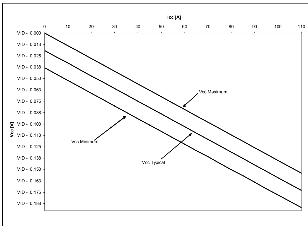
Figure 7-1. V_{CC} Static and Transient Tolerance Loadlines
